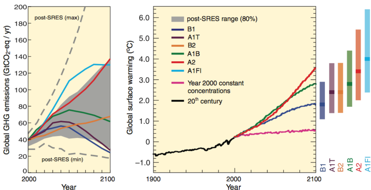
Figure A1. Scenarios for GHG emissions from 2000 to 2100 and projections of surface temperatures
